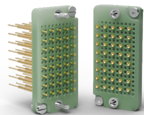
Signal block 40 pole
